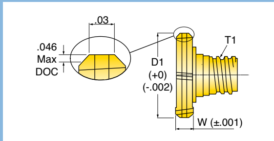
Slotting
