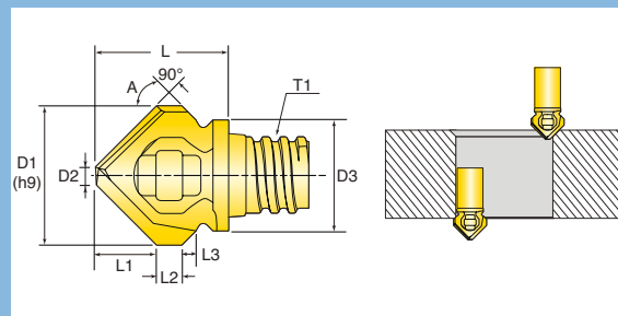
Countersink
